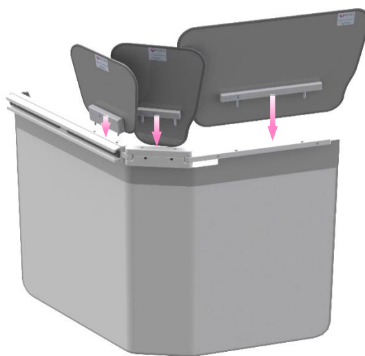
Lower body radiation shield – 312/E-020 (reverse side showing location of three optional top shields)
